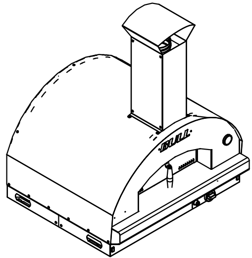
Isometric View
