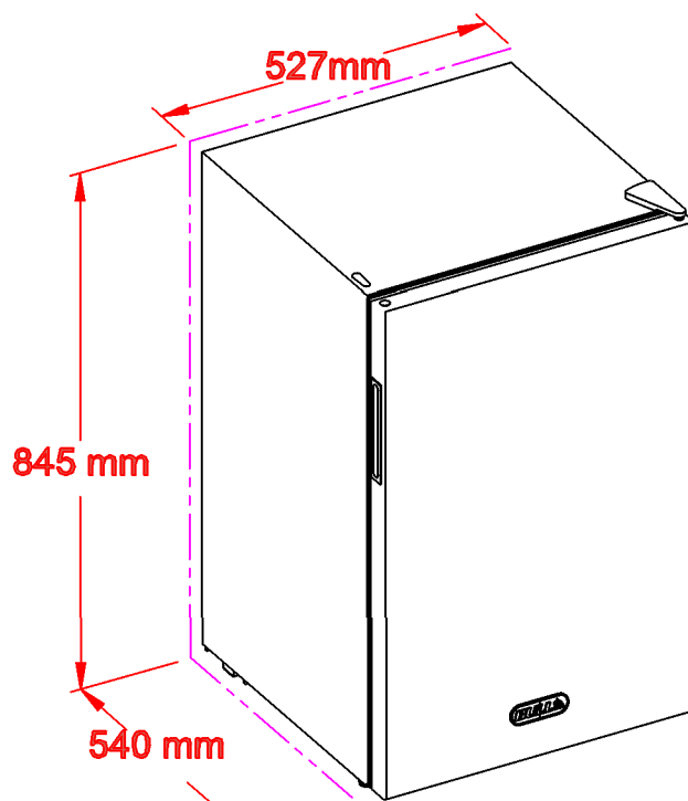
PERSPECTIVE VIEW WITH INSTALLATION CUT OUT DIMENSIONS (SEE NOTE 2 FOR VENTILATION REQUIREMENTS)
