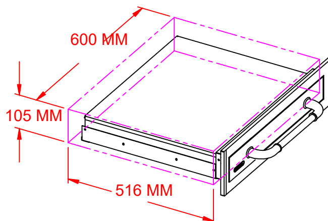
PERSPECTIVE VIEW WITH INSTALLATION CUT OUT DIMENSIONS
