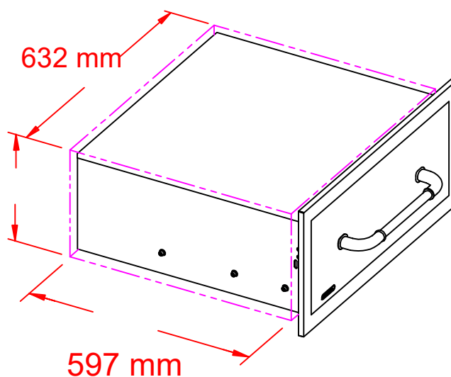
PERSPECTIVE VIEW WITH INSTALLATION CUT OUT DIMENSIONS
