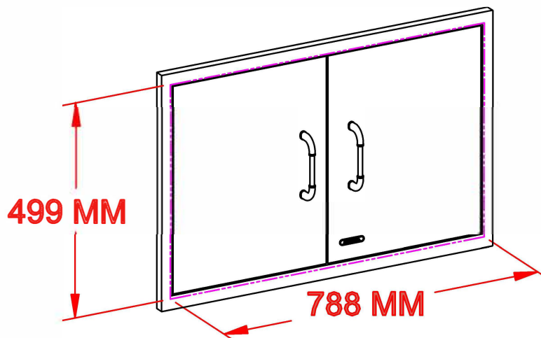
PERSPECTIVE VIEW WITH INSTALLATION CUT OUT DIMENSIONS
