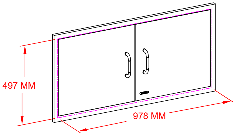
PERSPECTIVE VIEW WITH INSTALLATION CUT OUT DIMENSIONS
