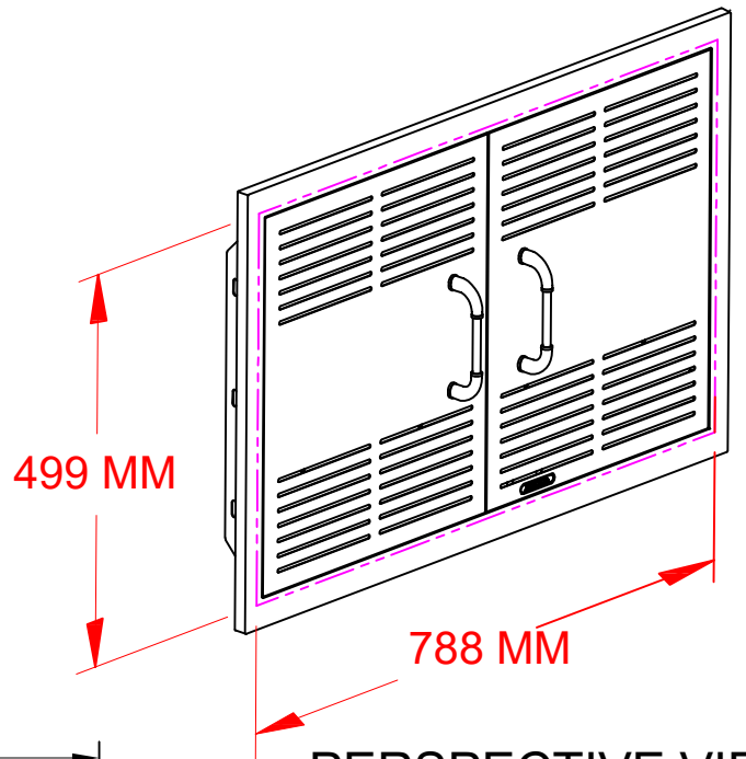
PERSPECTIVE VIEW WITH INSTALLATION CUT OUT DIMENSIONS
