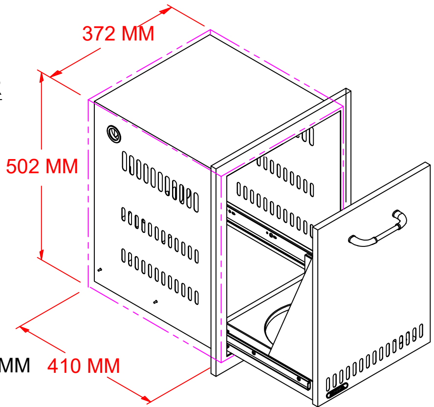
PERSPECTIVE VIEW WITH INSTALLATION CUT OUT DIMENSIONS
