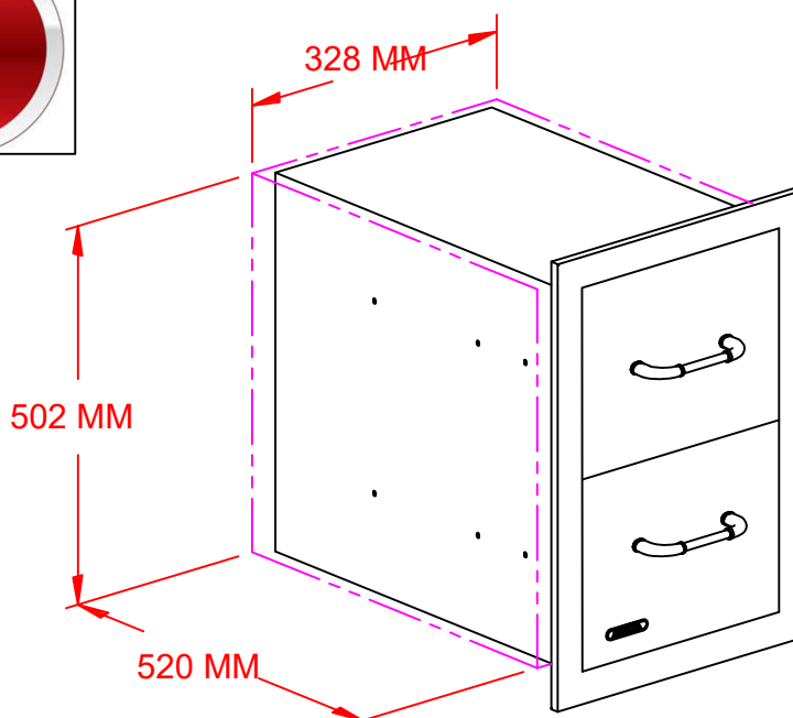
PERSPECTIVE VIEW WITH INSTALLATION CUT OUT DIMENSIONS
