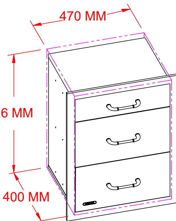
PERSPECTIVE VIEW WITH INSTALLATION CUT OUT DIMENSIONS
