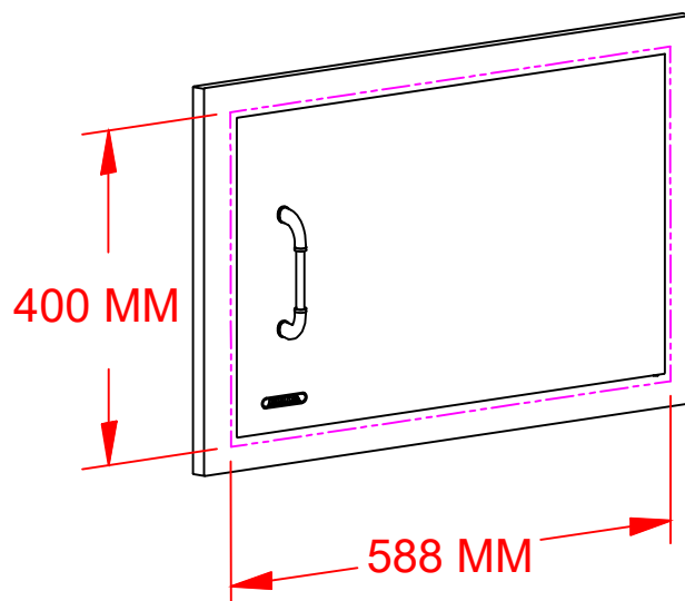
PERSPECTIVE VIEW WITH INSTALLATION CUT OUT DIMENSIONS
