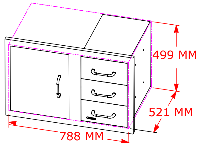
REVERSE PERSPECTIVE VIEW WITH INSTALLATION CUT OUT DIMENSIONS
