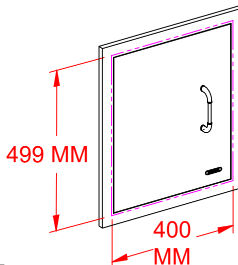
PERSPECTIVE VIEW WITH INSTALLATION CUT OUT DIMENSIONS
